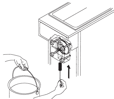
Figure N Clean Valve Body
