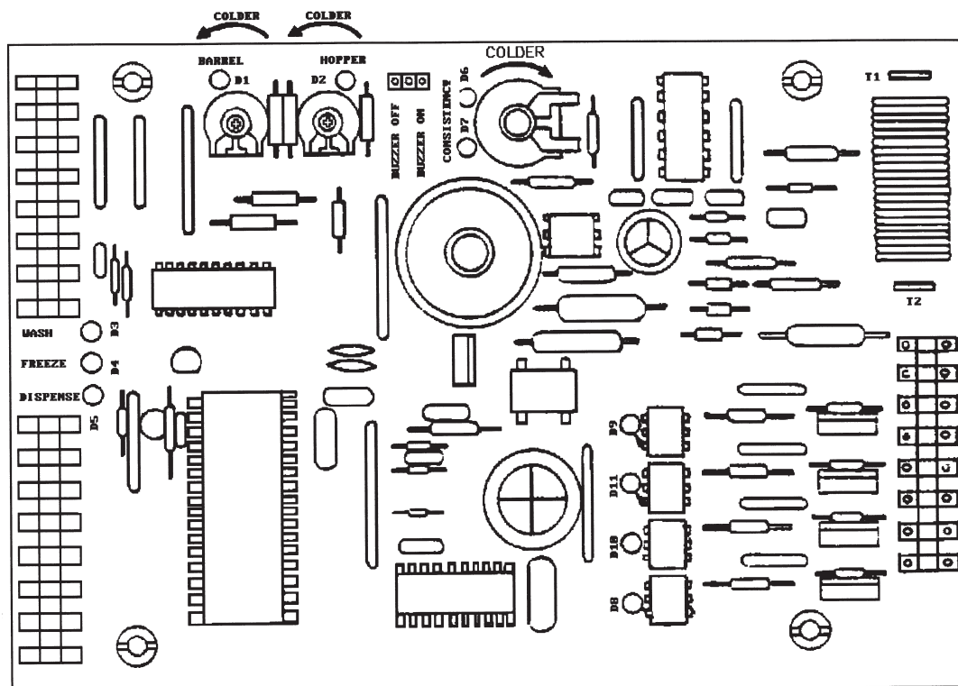
Figure I Electronic Control Board
