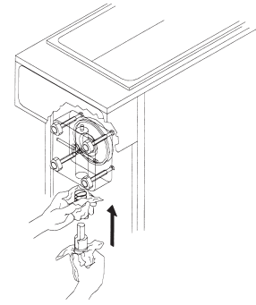
Figure Q Installing Plunger and Spring
