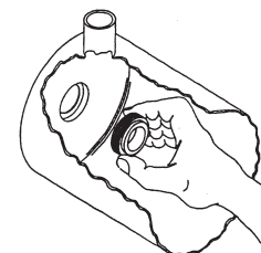
Figure V Installing the stationary half seal
