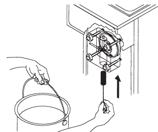
Figure T Clean Valve Body
