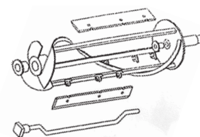
Figure W Dasher Assembly
