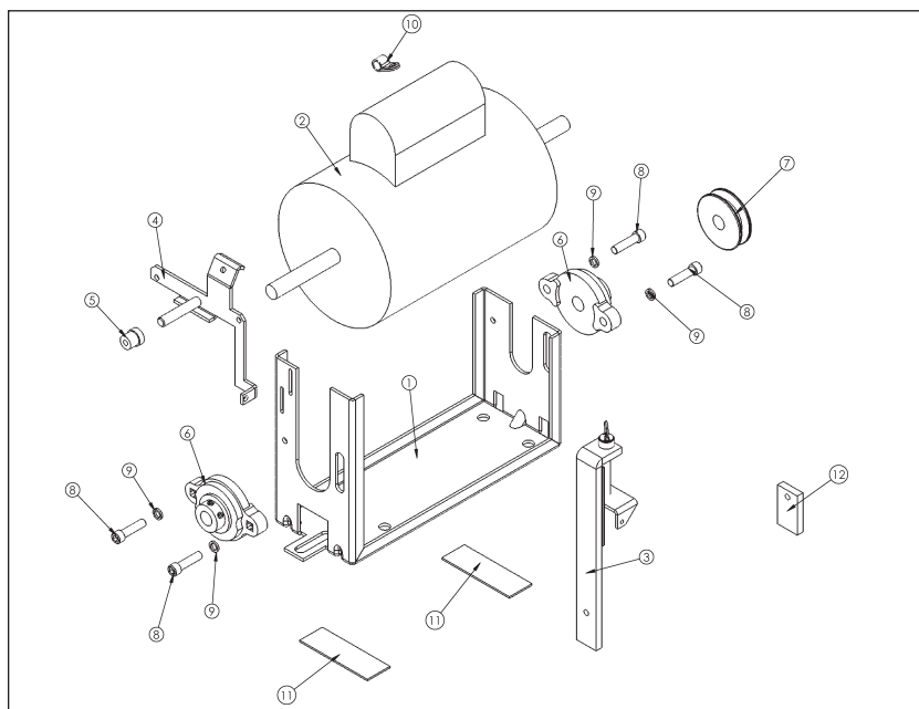
Drive Motor Assembly (See figure on left)
