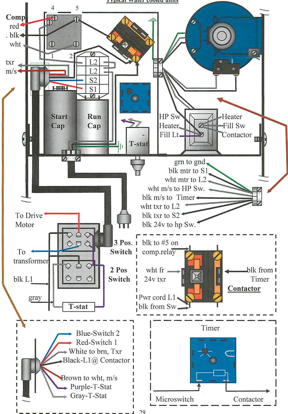
Typical Water cooled units
