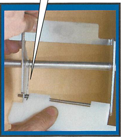
Step 1: Attach scraper blade spring F6517as shown.
